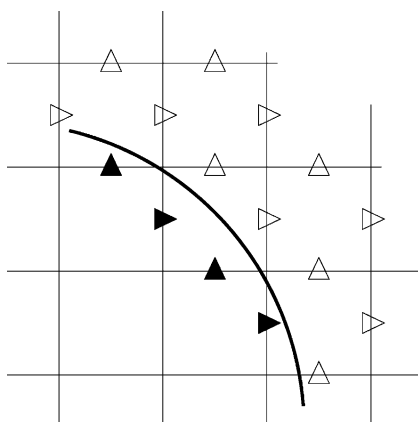
Fig. 6. Schematic of computational domain with an immersed boundary for two-dimensional staggered grid ( U , V components are located on the cell face). \triangleright , the location of U component in fluid domain; \blacktriangleright , the ghost cell location of U component; \triangle , the location of V component in fluid domain and \blacktriangle the ghost cell location of V component.
